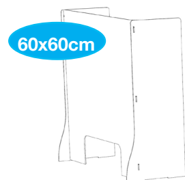
CA-0520_600-600 spit protection 612x600x250mm €140,- w/o taxes, excl. shipping
